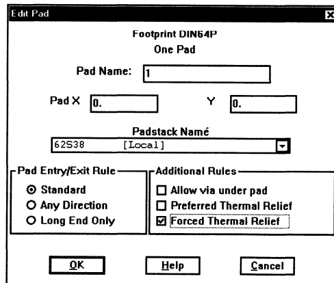
Specifying a forced thermal relief in the Edit Pad dialog box.
