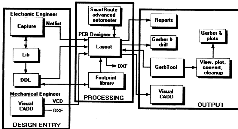
The printed circuit board design flow.
