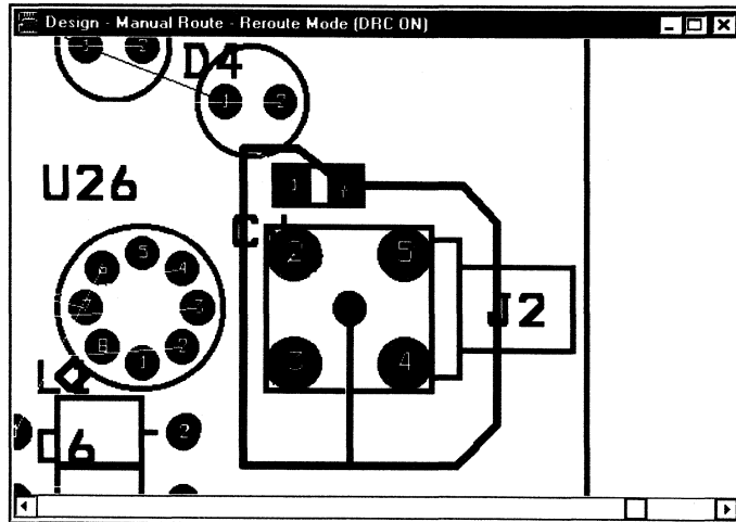
Creating a duplicate connection.
