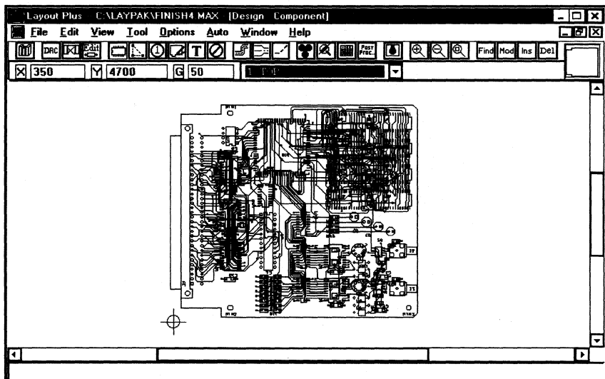
The Layout design window.
